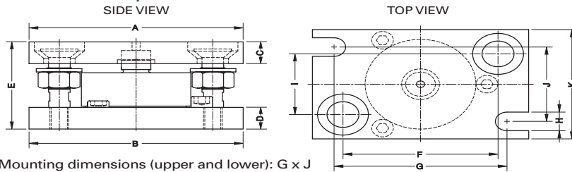
Mounting dimensions (upper and lower): G x J
